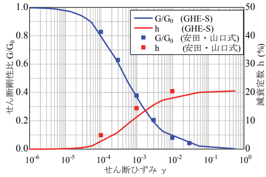
(b) No. 2層
