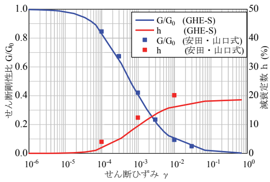
(a) No. 3層
