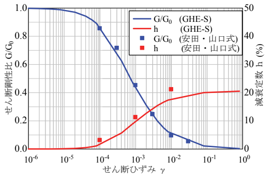
(c) No. 5層
