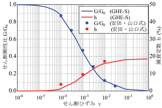
(a) No. 1層
